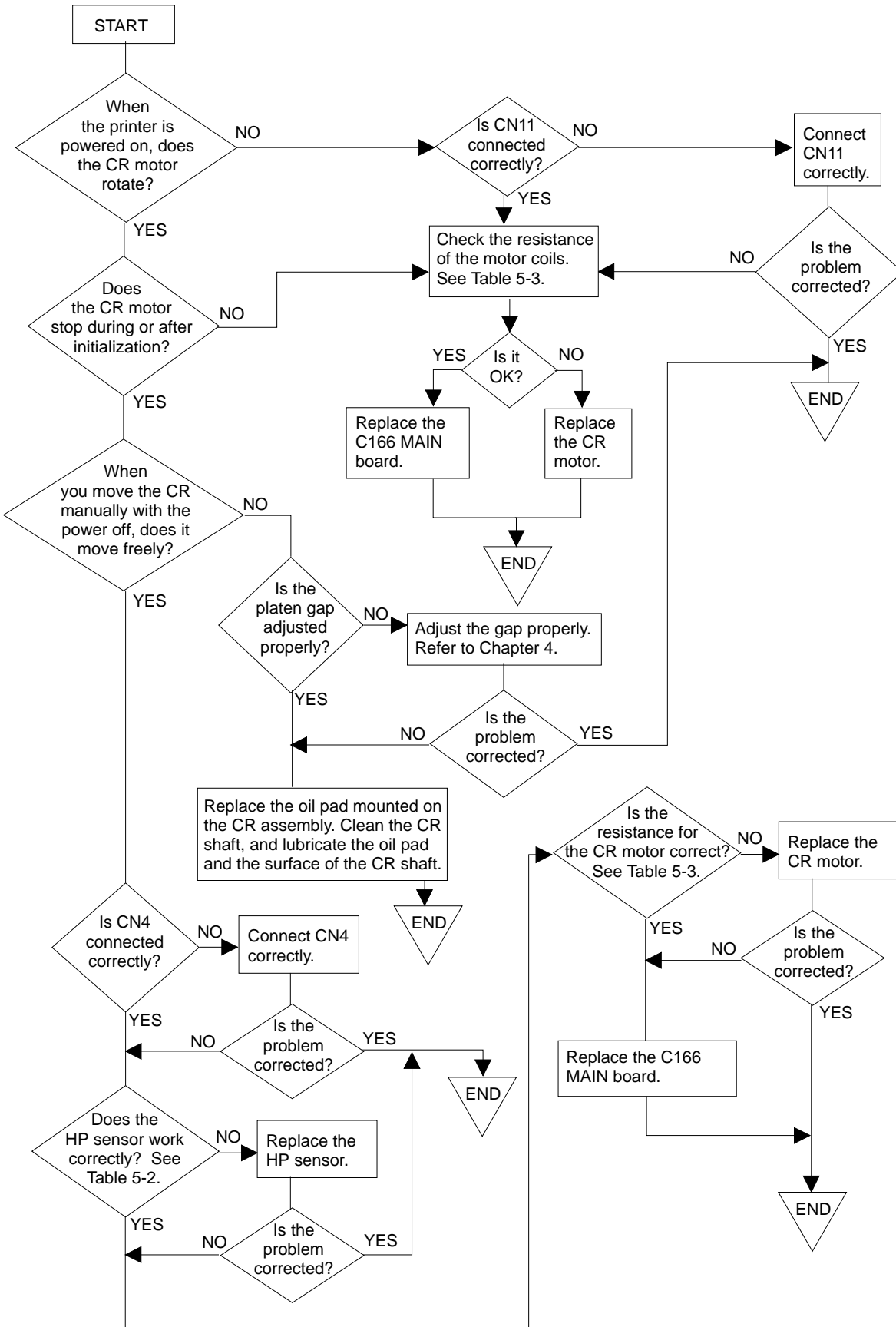
Figure 5-3 Flowchart 2
