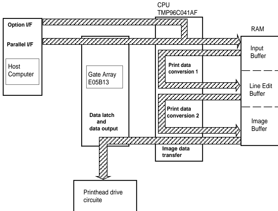
Figure 2-31 Data Flow
