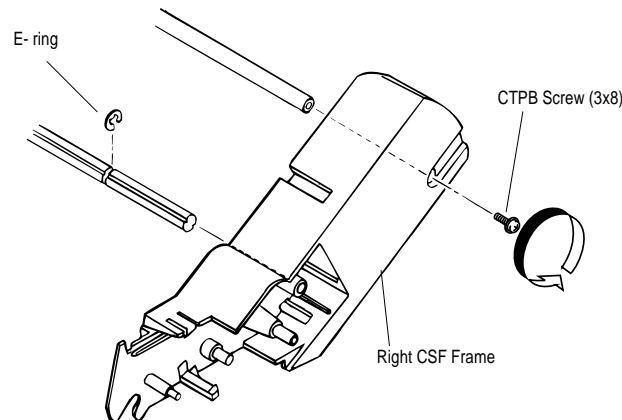
Figure 3-51 Removing 1 E-ring and 2 CTBS Screws
