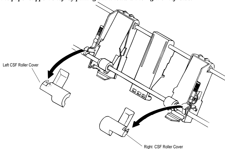
Figure 3-52 Removing the CSF Roller Cover
