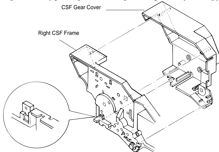
Figure 3-39 Releasing the Clips for the CSF Gear Cover
