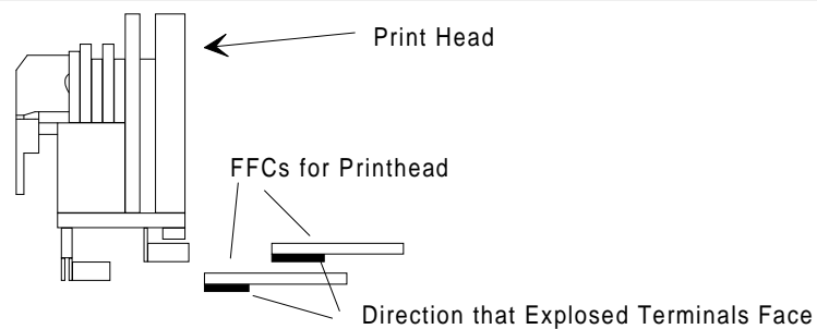
Figure 3-7 Method for Connecting the Printhead FFC
