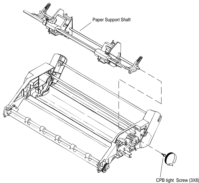
Figure 3-44 Removing the CBP Tight (3 x 8) Screw
