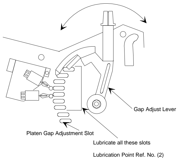
Figure 6-2. Lubrication Point 2
