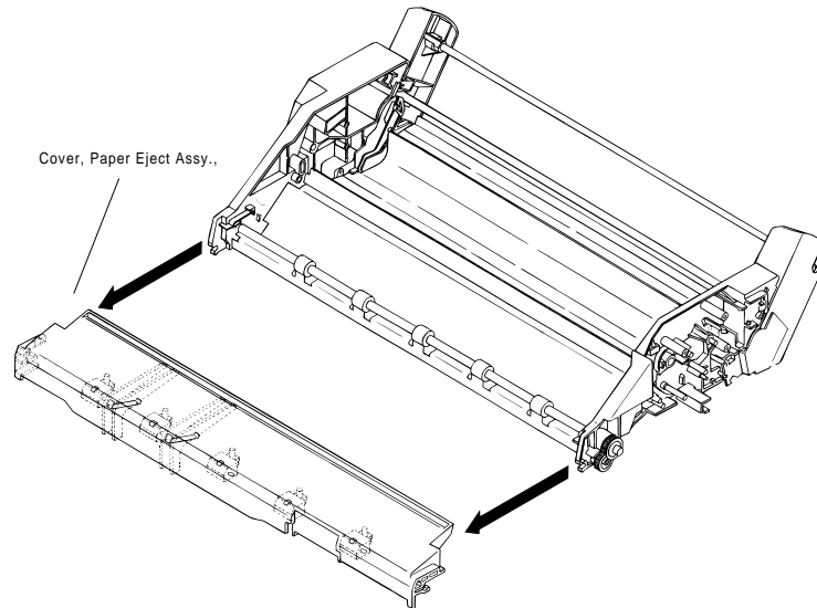
Figure 3-47 Removing the Paper Eject Assembly Cover
