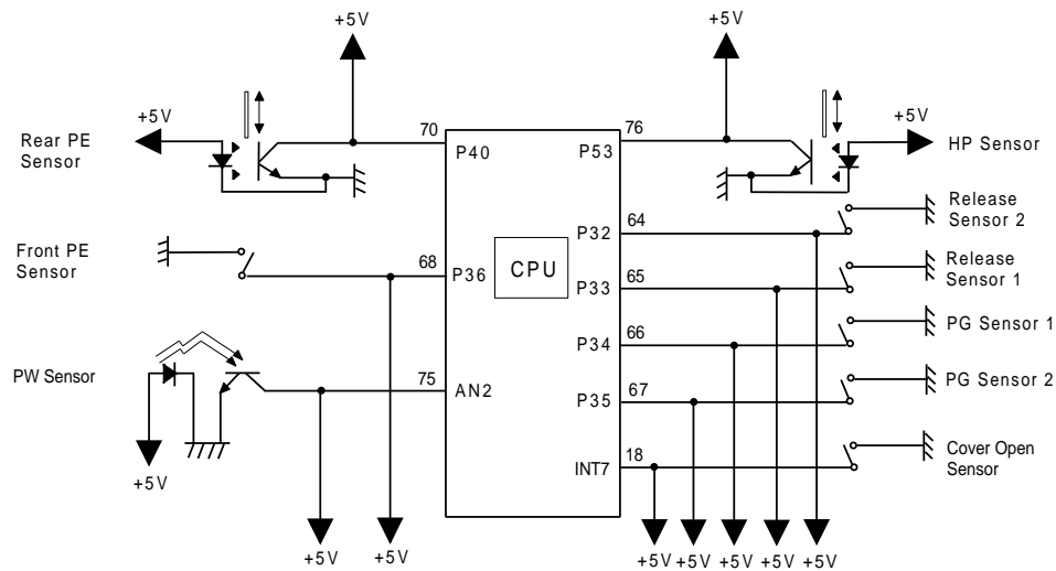
Figure 2-38 Sensor Circuits
