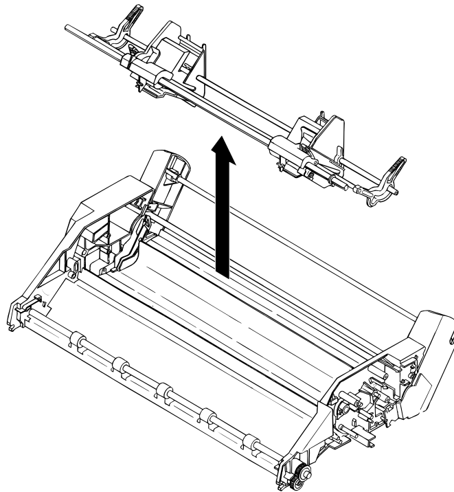
Figure 3-45 Removing the Paper Support Block Assembly
