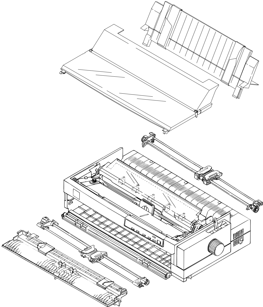
Figure 3-3 Before Starting Disassembly Procedures
