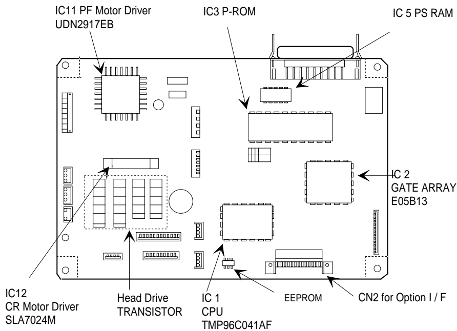
Figure 1-13 C165 MAIN Board Assembly
