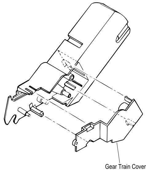
Figure 3-49 Removing the Gear Train Cover
