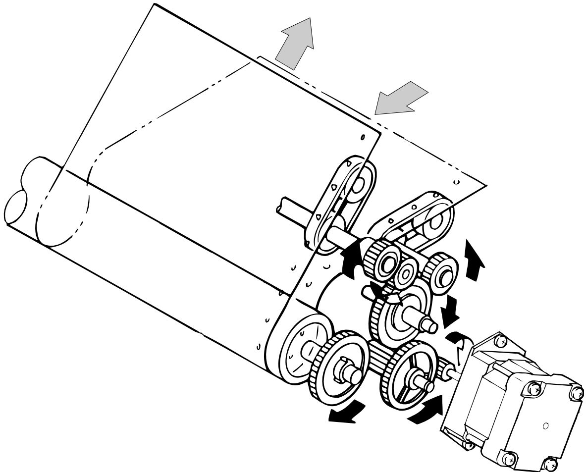
Figure. 2-9 Push-Pull Tractor Operation Using the Rear Paper Entrance
