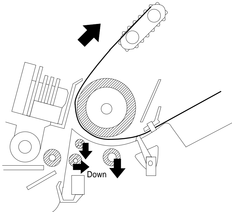
Figure. 2-14. Pull Tractor Feeding Using the Rear Entrance
