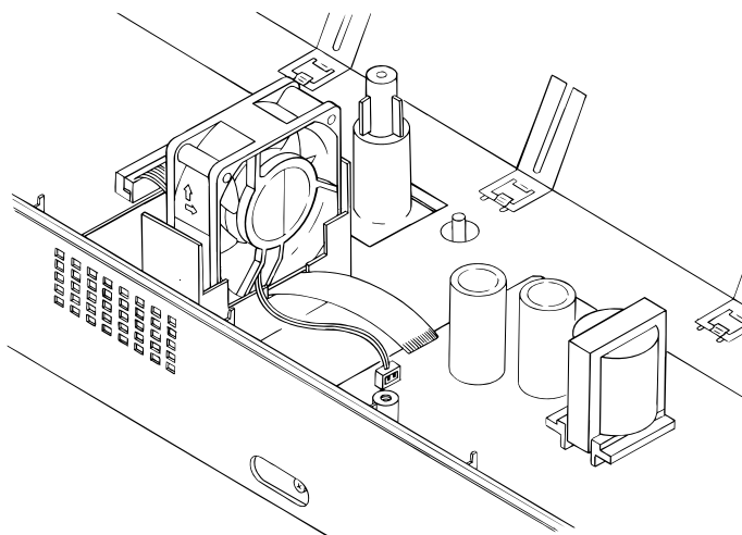
Figure 3-38 Direction for Mounting the Fan Motor
