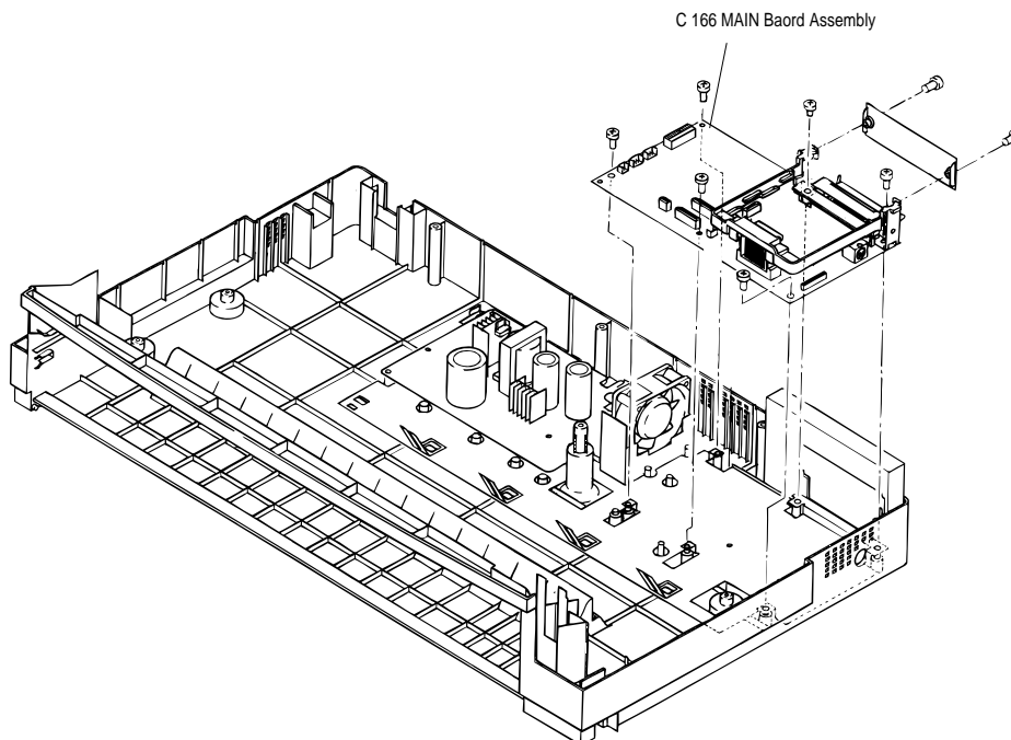
Figure 3-36 Removing the C165 MAIN Baord Assembly
