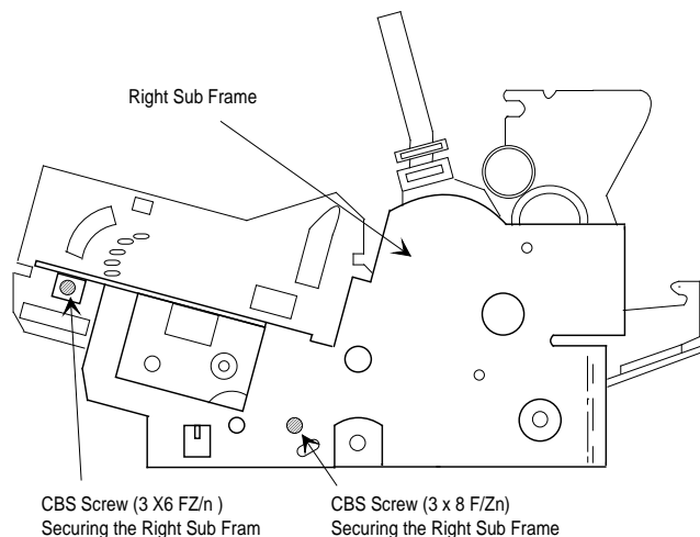
Figure 3-21 Removing the Right Sub Frame
