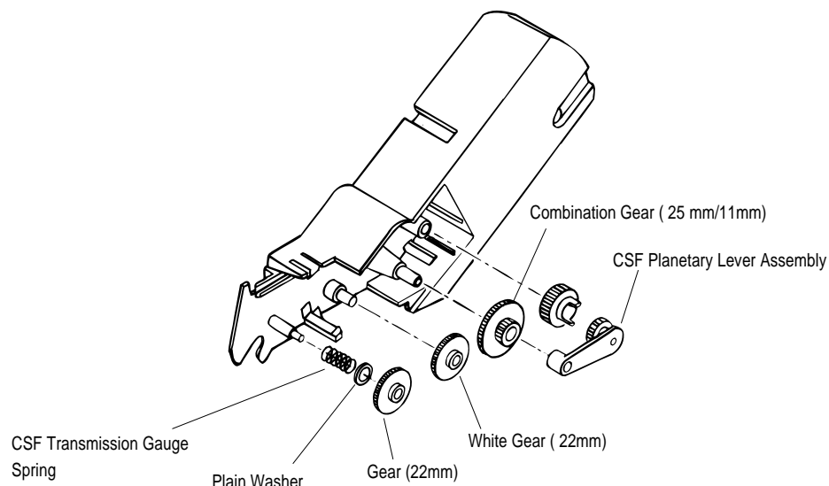
Figure 3-50 Engaging 5 Gears
