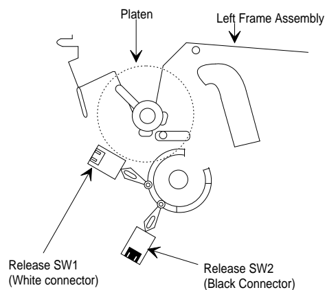
Figure 3-26 Cable Connections for the Release Lever Sensors
