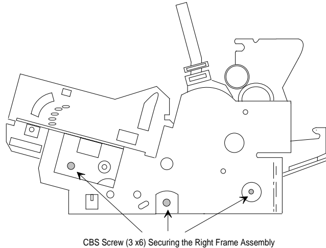
Figure 3-20 Removing the Right Frame Assembly
