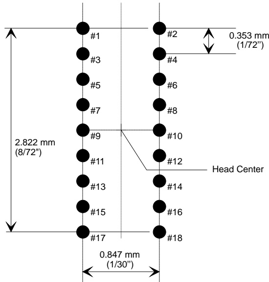
Figure 1-2. Pin Configuration
