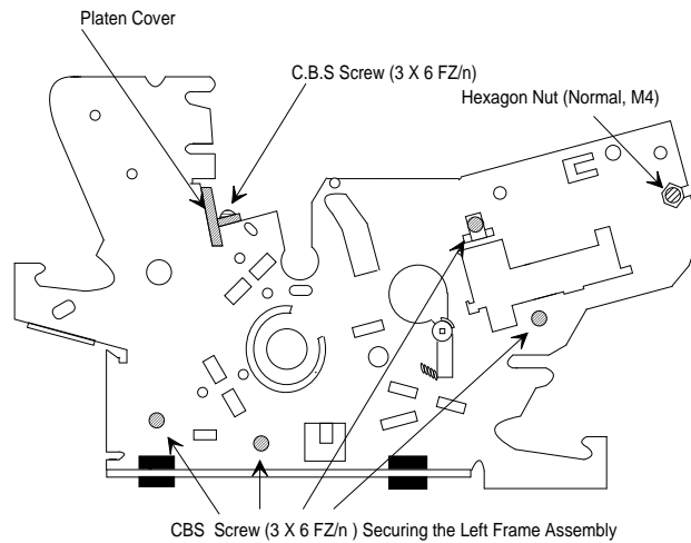
Figure 3-25 Removing the Left Frame Assembly
