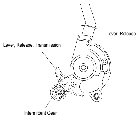
Figure 3-23 Engaging Gears 2
