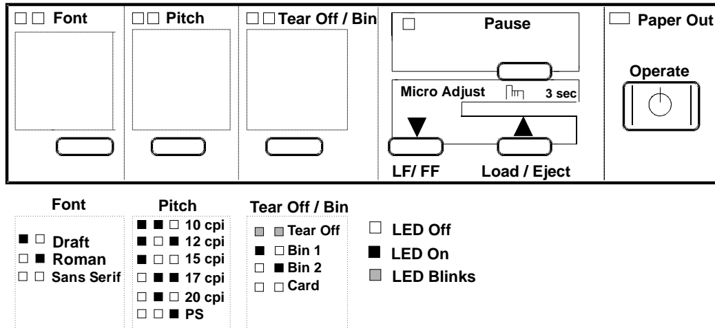
Figure 1-9 Control Panel
