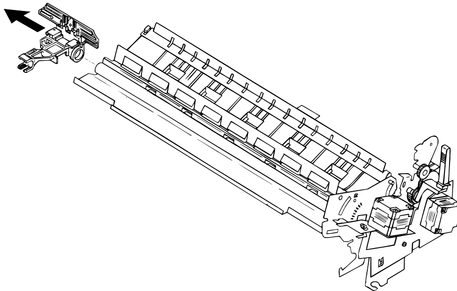
Figure 3-30 Removing the CR Assembly
