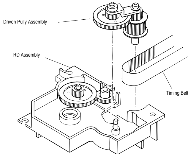
Figure 3-27 Removing the RD Assembly
