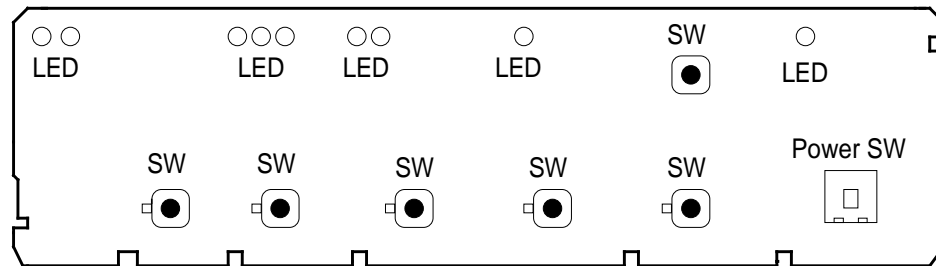
Figure 1-15 Board Assembly C165 PNL
