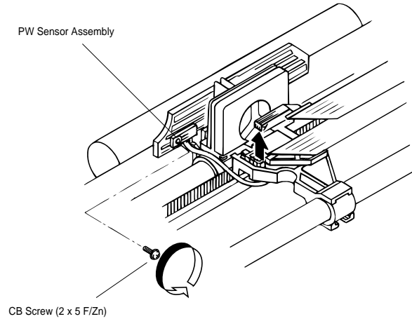
Figure 3-29 Disconnecting the FFCs
