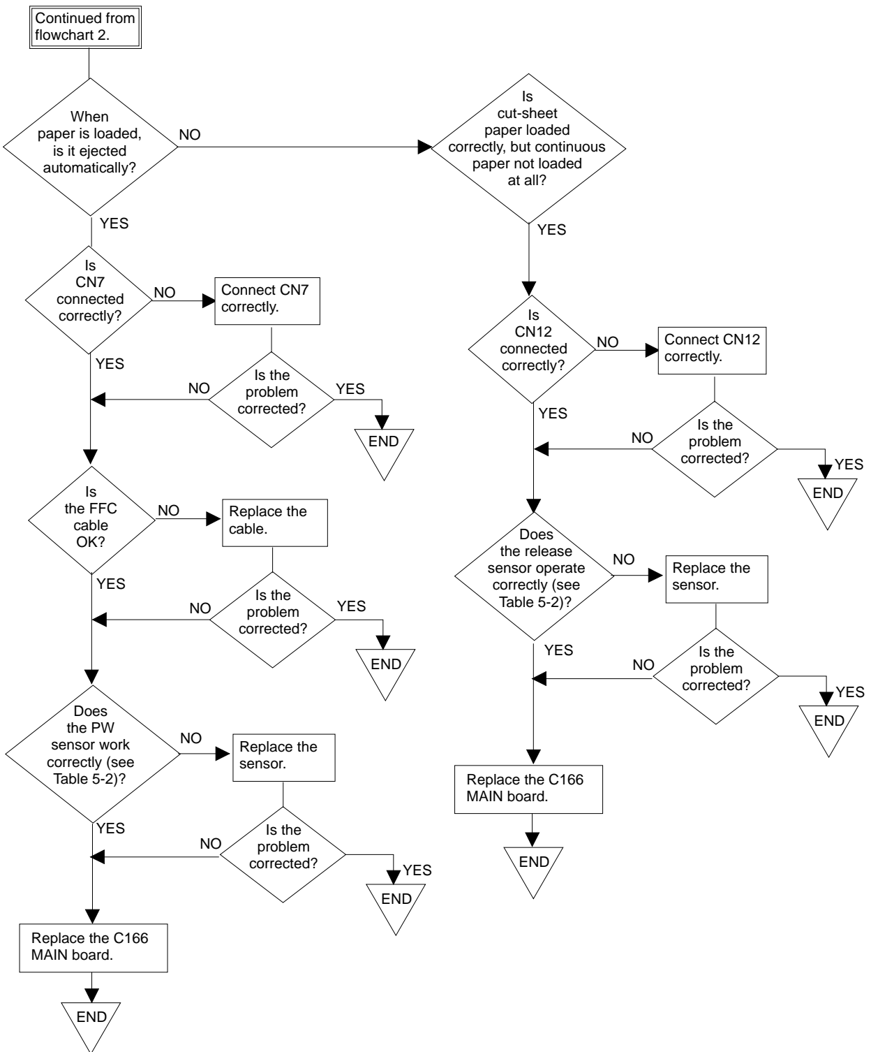
Figure 5-5 Flowchart 3
