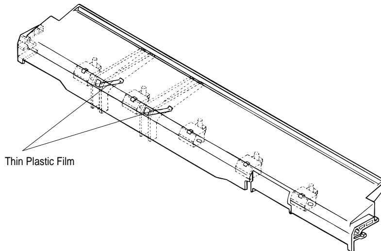
Figure 3-48 Assembling the Paper Eject Assembly Cover
