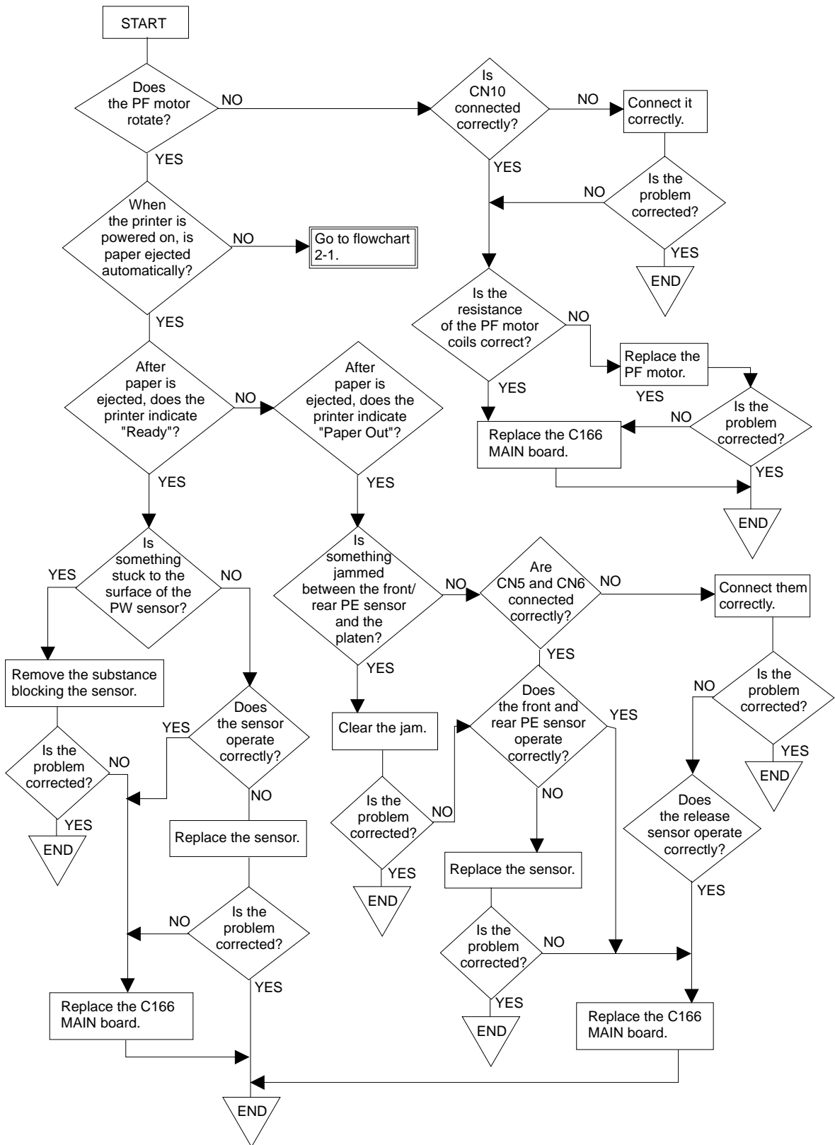
Figure 5-4 Flowchart 2-1
