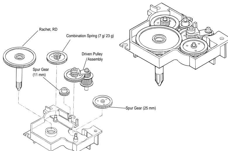
Figure 3-28 Engaging Gears for the RD Assembly
