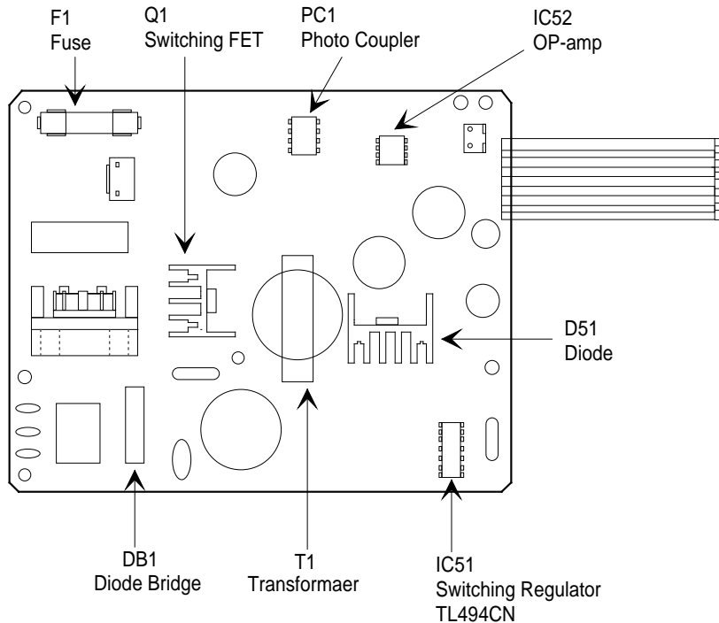
Figure 1-14 C165 PSB/PSE Board Assembly
