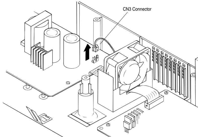
Figure 3-37 Removing the C165 PSB/E Board Assembly
