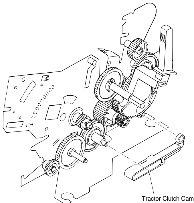
Figure 3-24 Engaging the Tractor Clutch Cam
