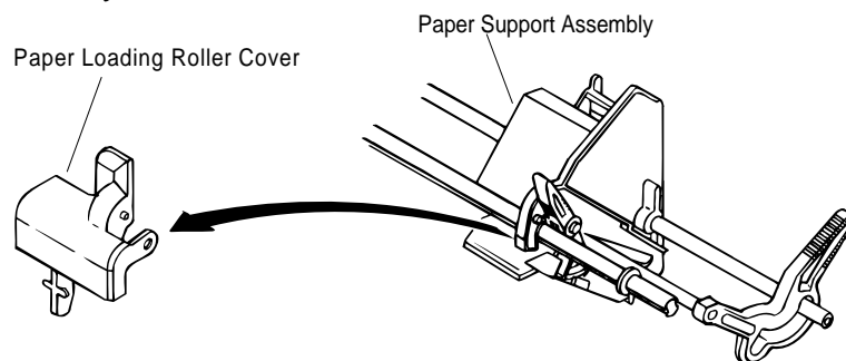
Figure 3-46 Removing the Paper Loading Roller Cover Assembly
