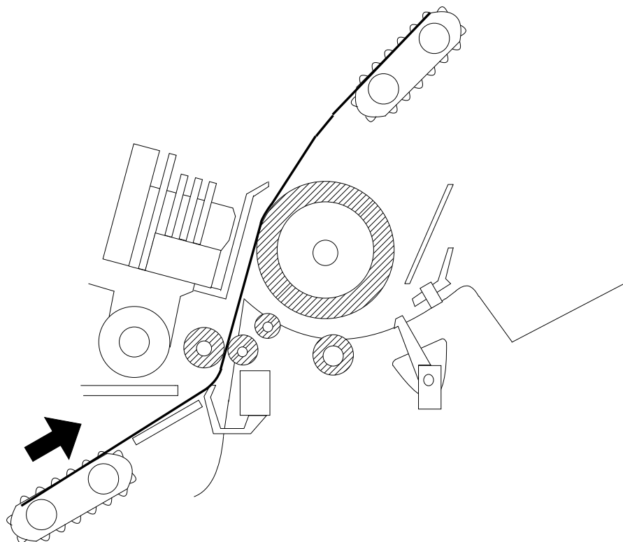
Figure 2-19 Pull Tractor Feeding Using the Front Entrance
