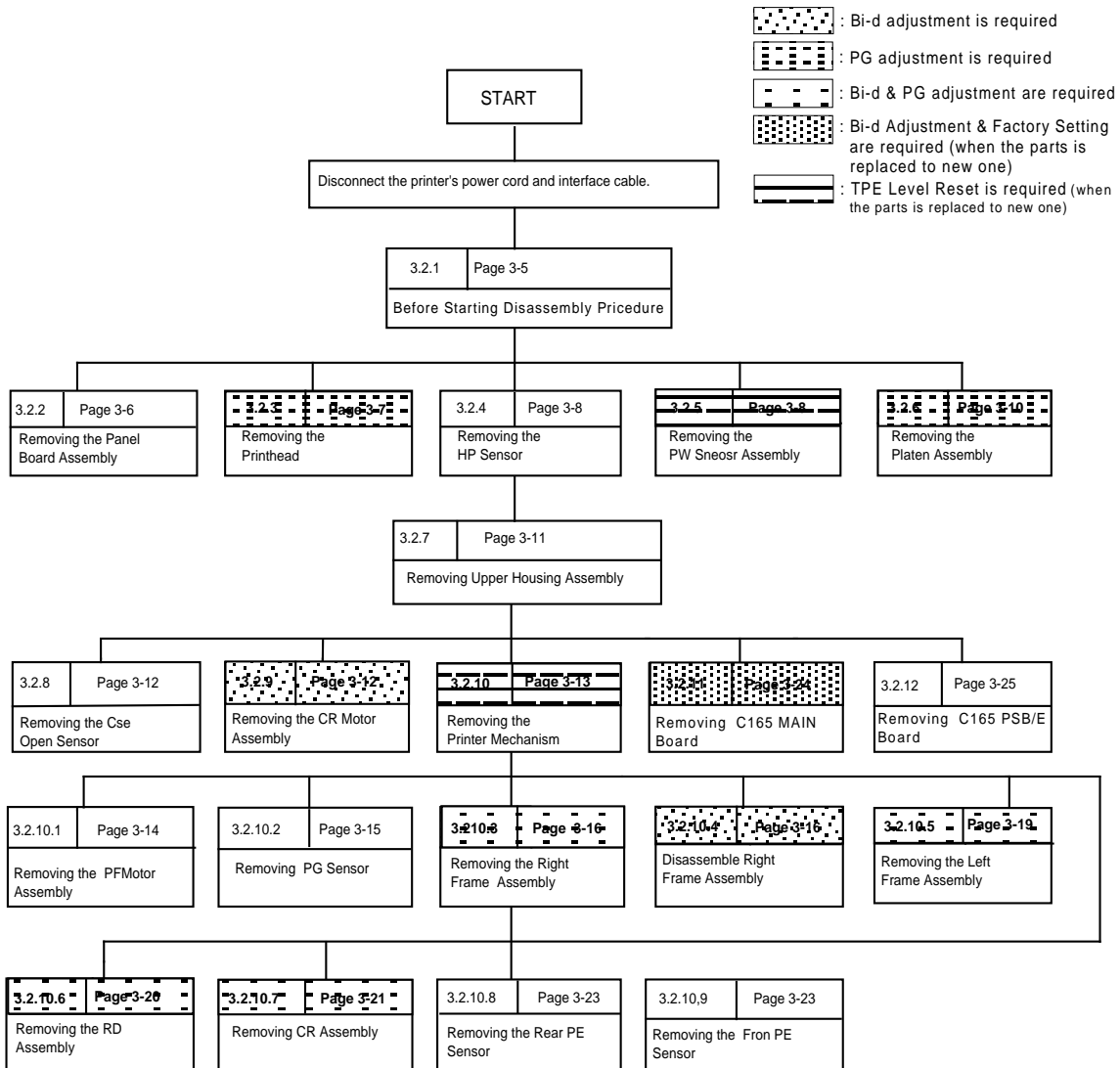
Figure 3-2 Flowchart for Disassembling the Printer
